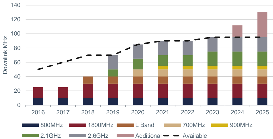
Figure A-13: Spectrum used by operator for LTE
