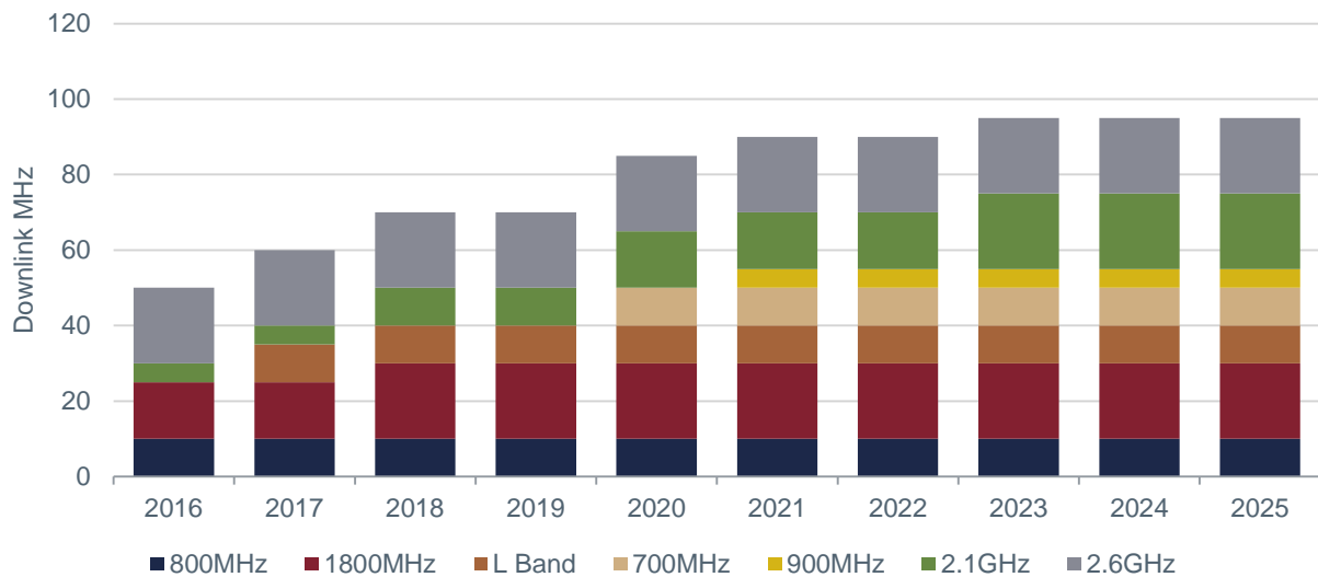
Figure A-5: Spectrum available for use by LTE
