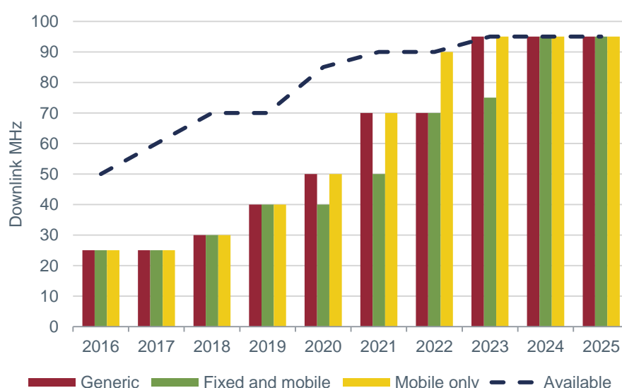
Figure 4-3: LTE/5G spectrum demand for downlink traffic – low traffic scenario
