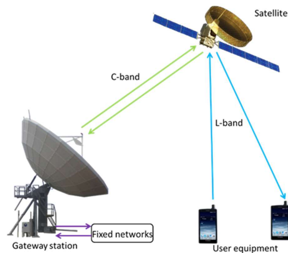
Figure 2.1: Mobile satellite communications system (green= feeder link, blue=user link).
